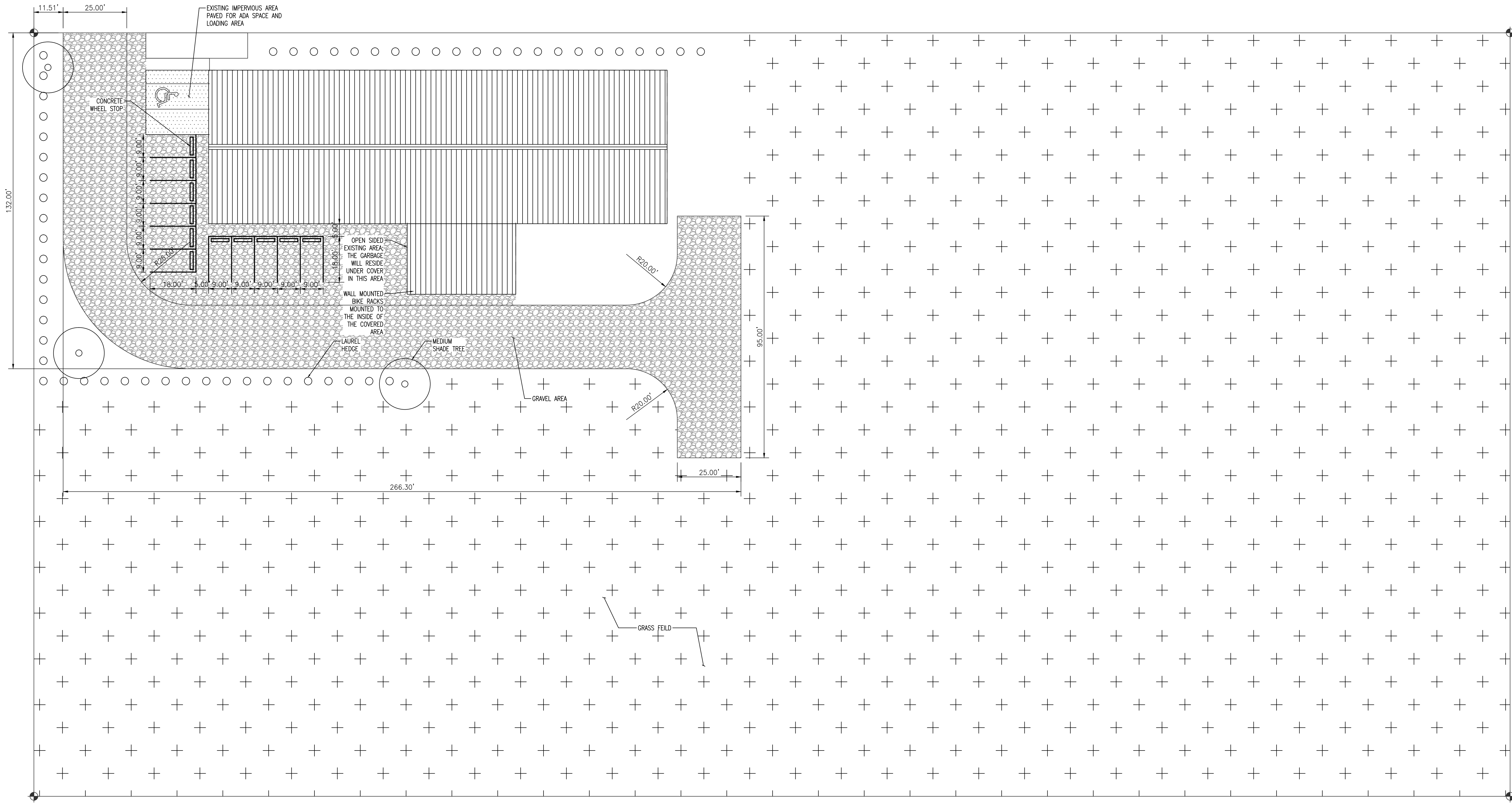
NORTH 1 SITE PLAN A10 1"=20'
